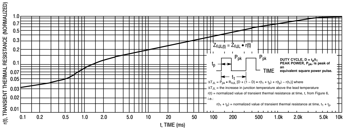
Figure 6. Thermal Response
