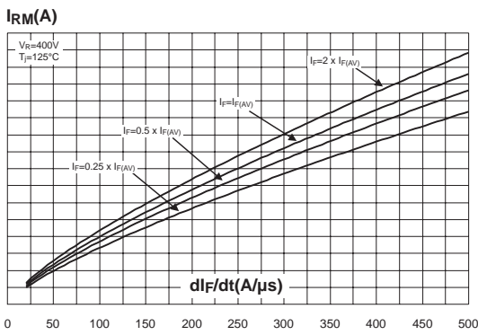
Fig. 4: Peak reverse recovery current versus di_F/dt (typical values).
