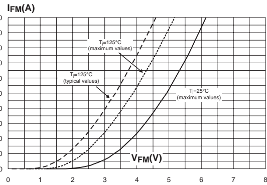
Fig. 2: Forward voltage drop versus forward current.
