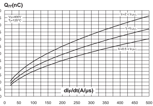
Fig. 6: Reverse recovery charges versus di_F/dt (typical values).
