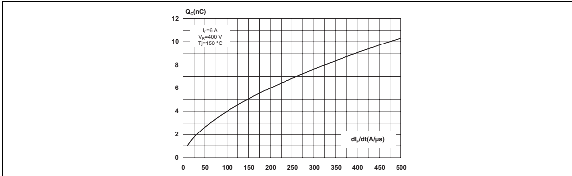
Figure 7. Total capacitive charges versus di_F/dt (typical values)
