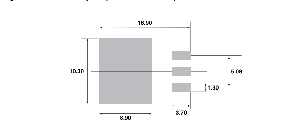
Figure 11. D 2 PAK footprint (dimensions in mm)
