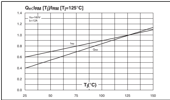
Figure 9. Dynamic parameters versus junction temperature
