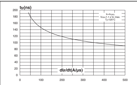
Figure 10. Forward recovery time versus di_F/dt (typical values)
