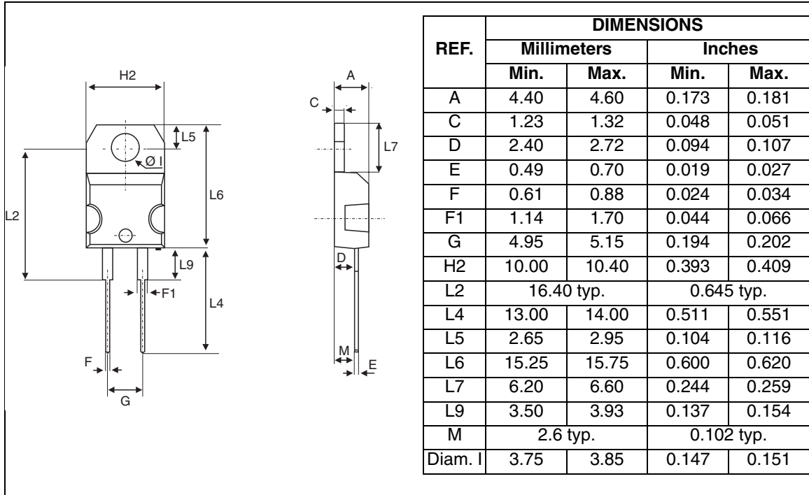
Figure 17: TO-220AC Package Mechanical Data
