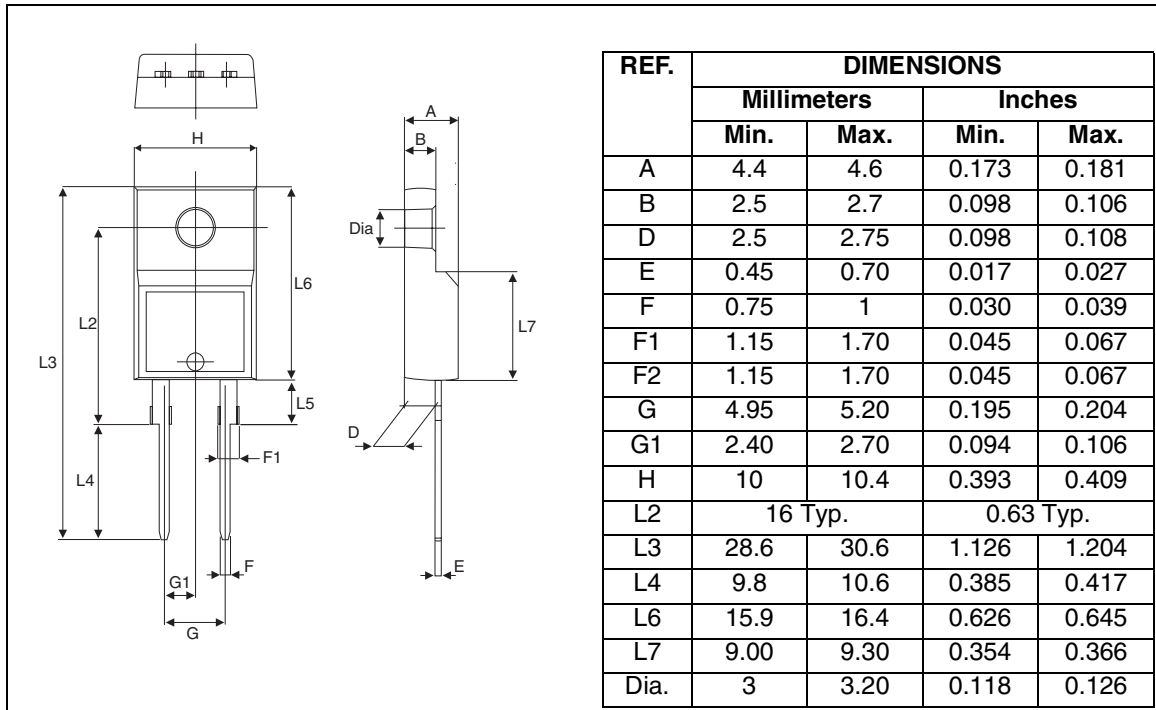
Figure 16: TO-220FPAC Package Mechanical Data
