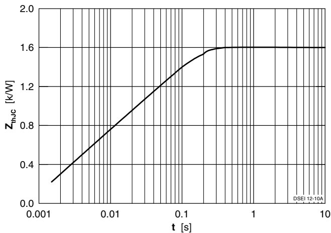
Fig. 7 Transient thermal resistance junction to case
