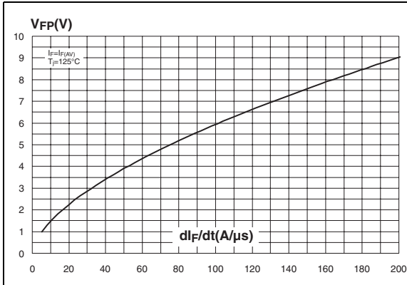
Figure 11. Transient peak forward voltage versus di_F/dt (90% confidence)
