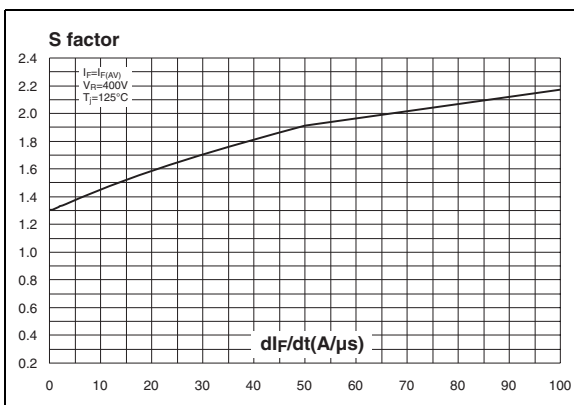
Figure 9. Softness factor versus di_F/dt (typical values)
