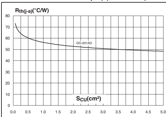
Figure 15. Thermal resistance junction to ambient versus copper surface under each lead (epoxy printed circuit board FR4, copper thickness: 35μm) (DO-201AD)
