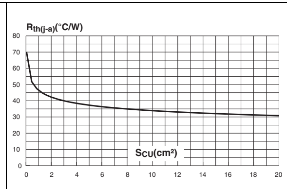
Figure 14. Thermal resistance junction to ambient versus copper surface under tab (epoxy FR4, eCU = 35 μm) (DPAK)
