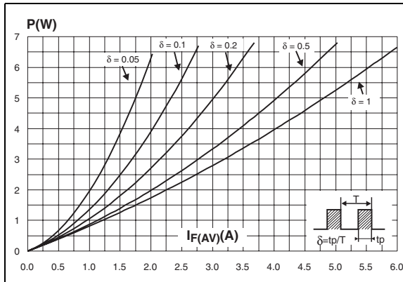
Figure 1. Conduction losses versus average current
