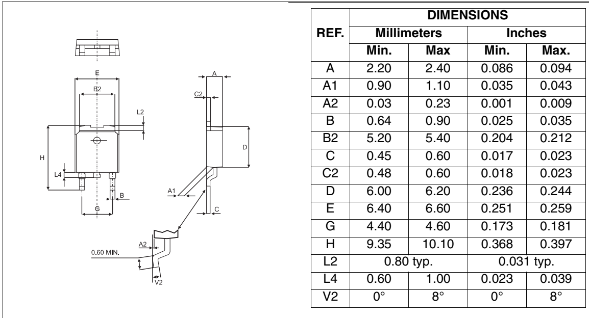
Figure 16: DPAK Package Mechanical Data
