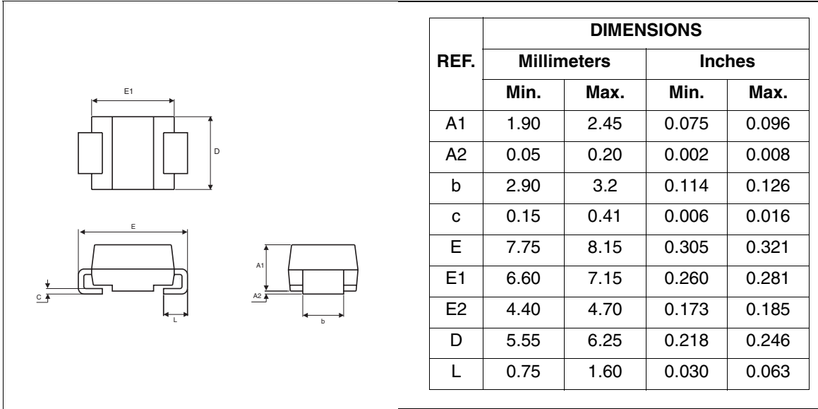
Figure 20: SMC Package Mechanical Data
