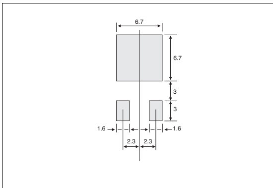
Figure 17: DPAK Foot Print Dimensions (in millimeters)
