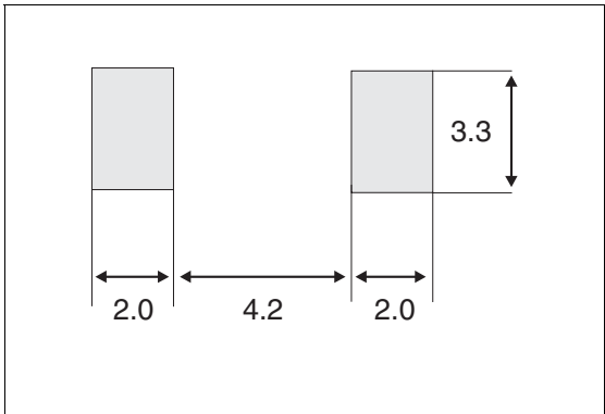
Figure 21: SMC Foot Print Dimensions (in millimeters)
