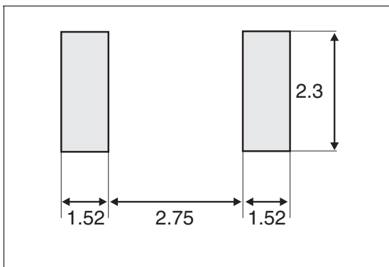
Figure 19: SMB Foot Print Dimensions (in millimeters)
