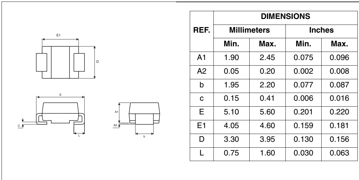
Figure 18: SMB Package Mechanical Data
