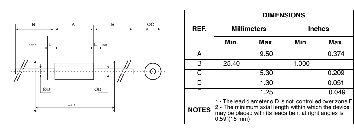
Figure 22: DO-201AD Package Mechanical Data
