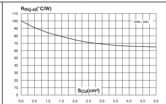
Figure 18. Thermal resistance junction to ambient versus copper surface under each lead (epoxy printed board FR4, e_{CU} = 35 \mu\text{m} ) (SMB / SMC)
