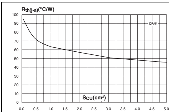
Figure 17. Thermal resistance junction to ambient versus copper surface under each lead (epoxy printed board FR4, e_{CU} = 35 \mu\text{m} ) (DPAK)
