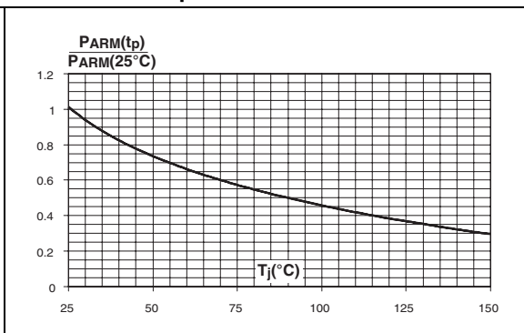
Figure 8. Normalized avalanche power derating versus junction temperature
