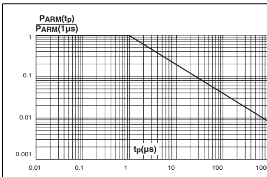
Figure 7. Normalized avalanche power derating versus pulse duration
