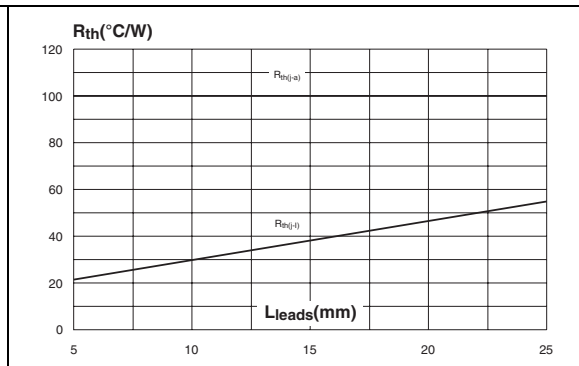
Figure 16. Thermal resistance versus lead length (DO-41)
