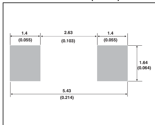
Figure 18. SMA footprint dimensions in millimeters (inches)
