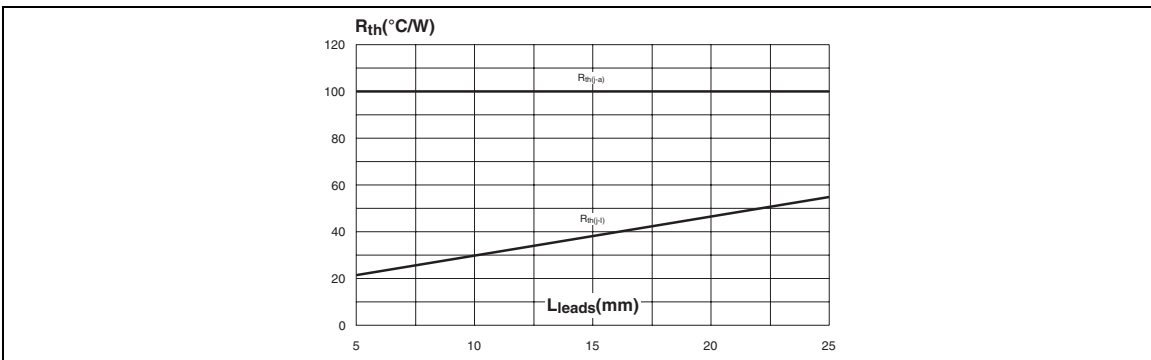
Figure 17. Thermal resistance versus lead length (DO-15)
