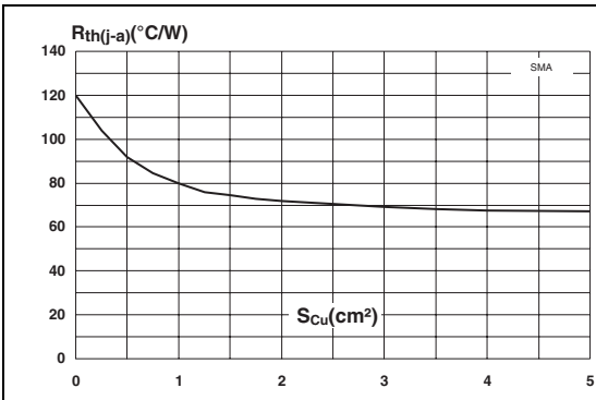
Figure 15. Thermal resistance junction to ambient versus copper surface under each lead - epoxy printed circuit board FR4, copper thickness = 35 μm (SMA)
