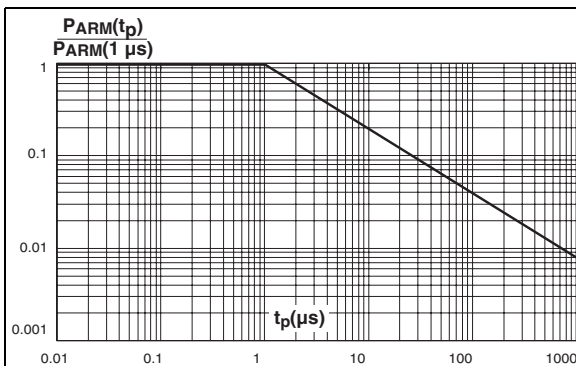
Figure 5. Normalized avalanche power derating versus pulse duration
