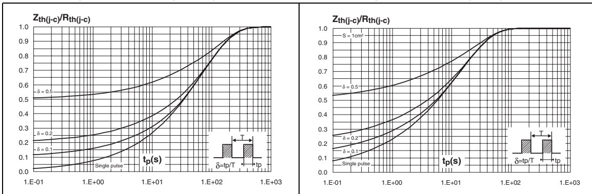
Figure 3. Relative variation of thermal impedance junction to case vs pulse duration (DO-41) Figure 4. Relative variation of thermal impedance junction to case vs pulse duration (SMA)
