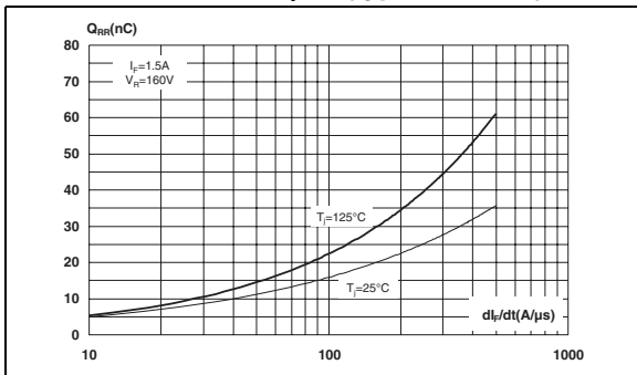
Figure 9. Reverse recovery charges versus diF/dt (typical values)
