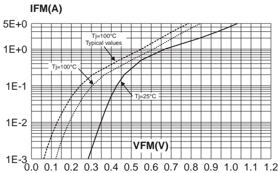
Fig. 8-2: Forward voltage drop versus forward current (maximum values).(STPS0560Z)
