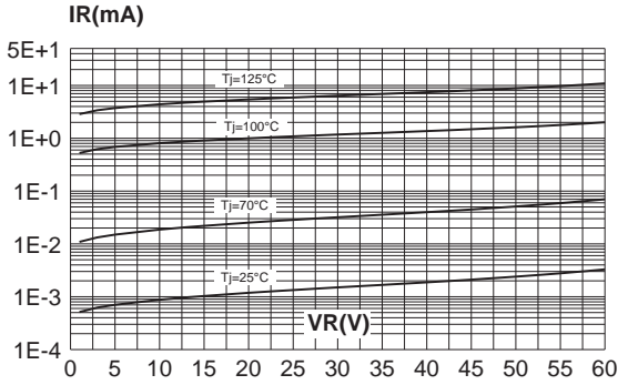
Fig. 5-2: Reverse leakage current versus reverse voltage applied (typical values).(STPS0560Z)
