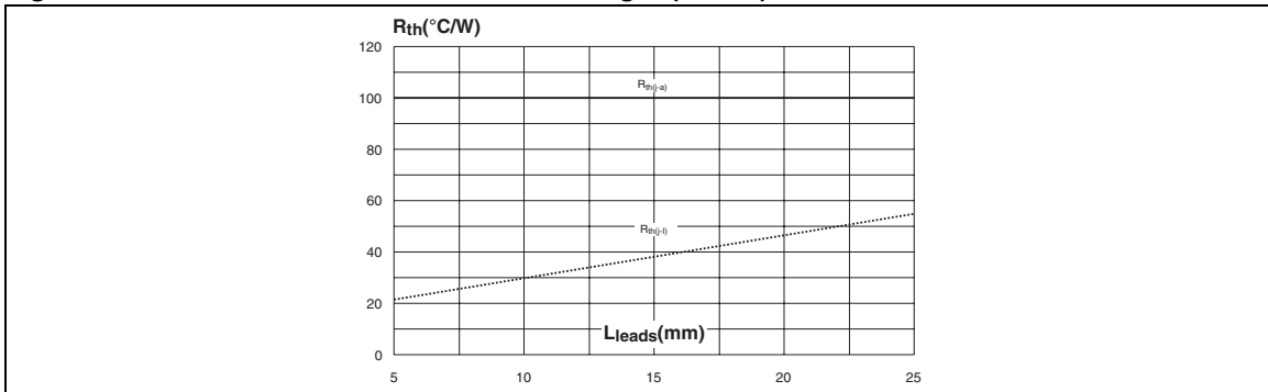
Figure 19. Thermal resistance versus lead length (DO-41)
