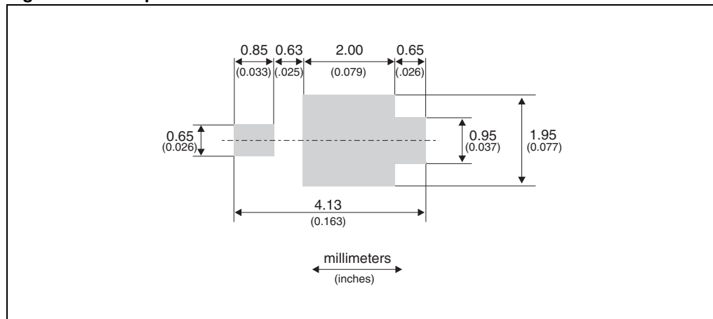
Figure 21. Footprint dimensions
