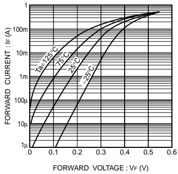
Fig. 1 Forward characteristics
