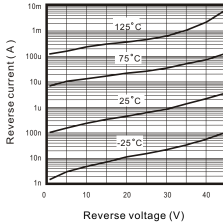
Fig. 2 - Reverse characteristics
