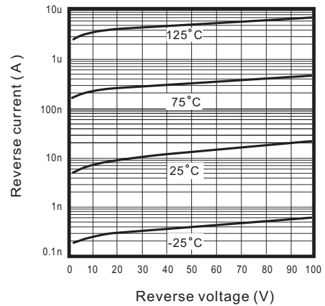
Fig. 2 - Reverse characteristics
