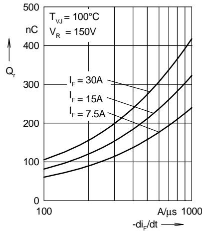
Fig. 2 Reverse recovery charge Q_r
