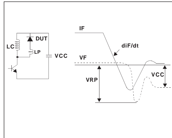
Fig. 14: Turn-off switching characteristics (with serie inductance).
