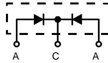
TO-247 AD
