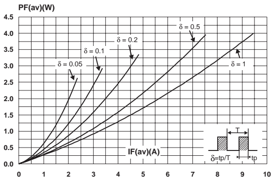
Fig. 1: Conduction losses versus average current.
