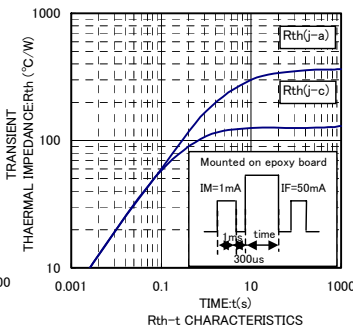
Rth-t CHARACTERISTICS
