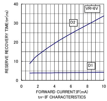
trr-IF CHARACTERISTICS
