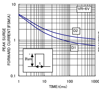
IFSM-t CHARACTERISTICS
