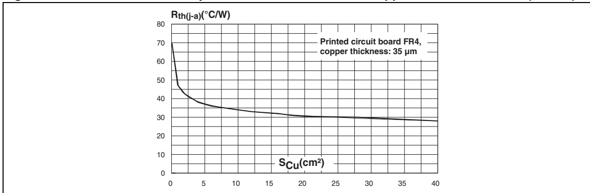
Figure 11. Thermal resistance, junction to ambient, versus copper surface under tab (D 2 PAK)
