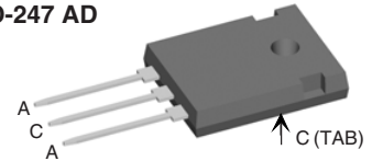
TO-247 AD
