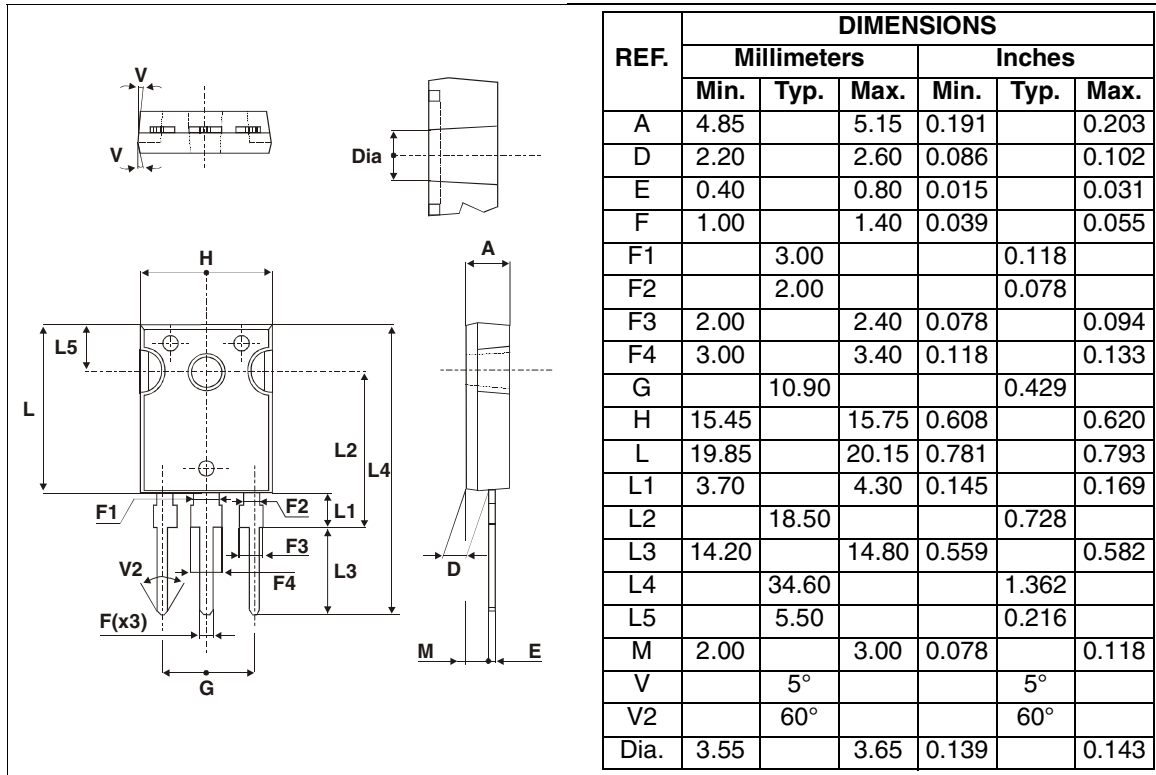
Figure 11: TO-247 Package Mechanical Data
