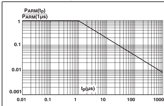
Figure 4. Normalized avalanche power derating vs. pulse duration
