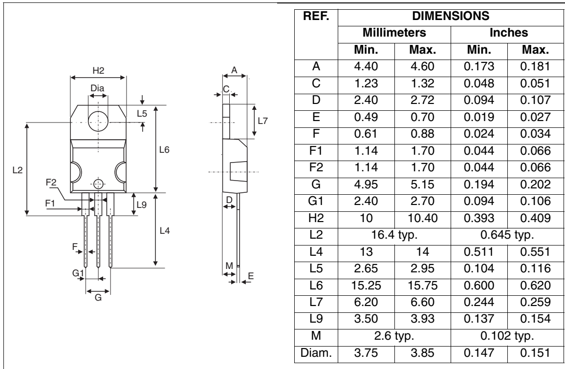
Figure 10: TO-220AB Package Mechanical Data
