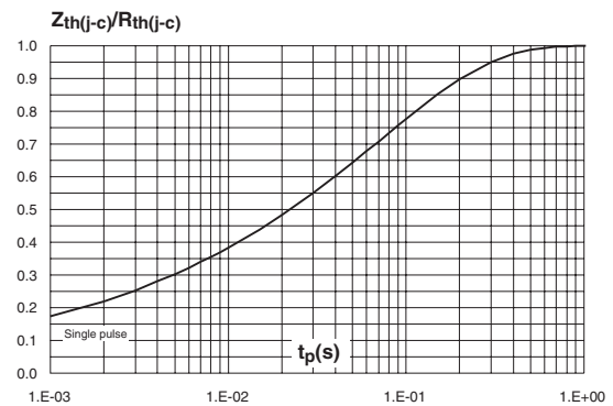
Figure 6: Relative variation of thermal impedance to case versus pulse duration (per diode)
