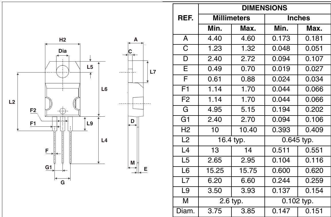
Figure 11: TO-220AB Package Mechanical Data
