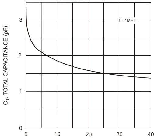
Fig. 3 Typical Capacitance
