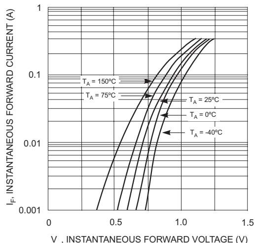
Fig. 2 Forward Characteristics
