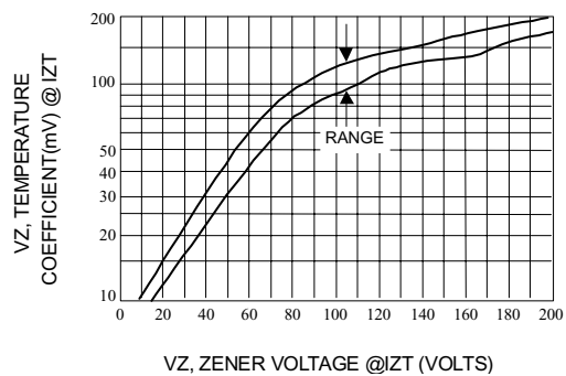
Fig. 6-UNITS 10 TO 200 VOLTS
