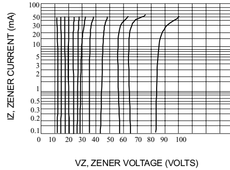
Fig. 8-V Z = 12 THRU 82 VOLTS
