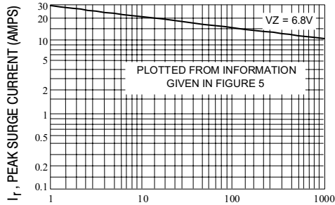
Fig. 6-PEAK SURGE CURRENT VERSUS PULSE WIDTH(SEE NOTE 3)
