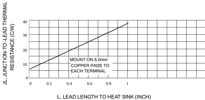
Fig. 4-TYPICAL THERMAL RESISTANCE
