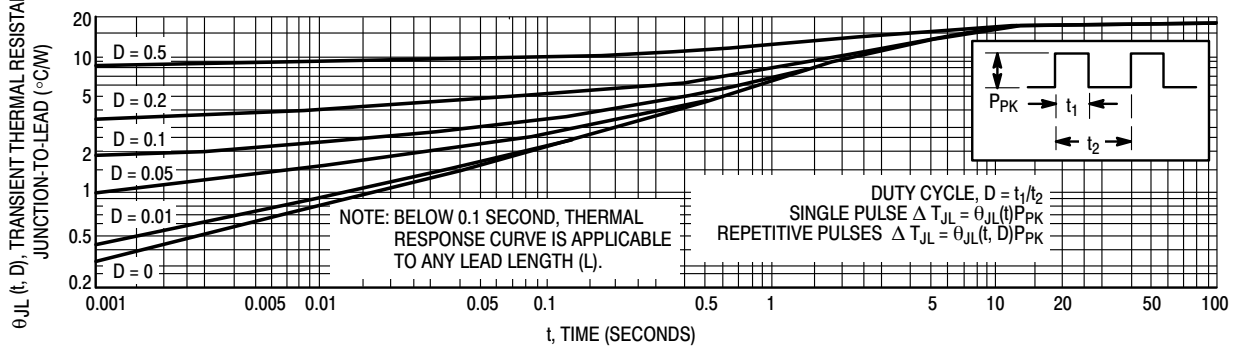
Figure 3. Typical Thermal Response L, Lead Length = 3/8 Inch
