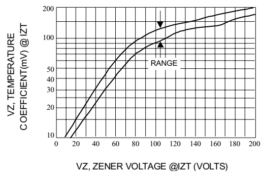
Fig. 6-UNITS 10 TO 200 VOLTS
