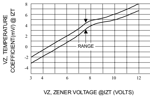
Fig. 5-UNITS 3.9 TO 12 VOLTS
