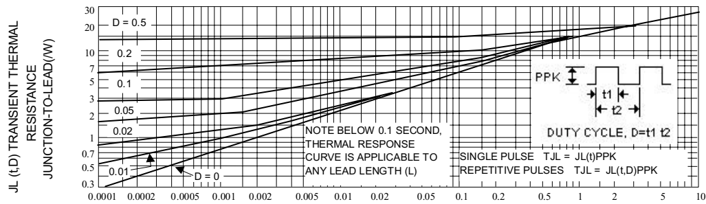
Fig. 2-TYPICAL THERMAL RESPONSE
