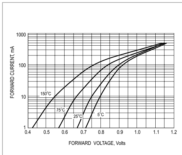
TYPICAL FORWARD VOLTAGE
