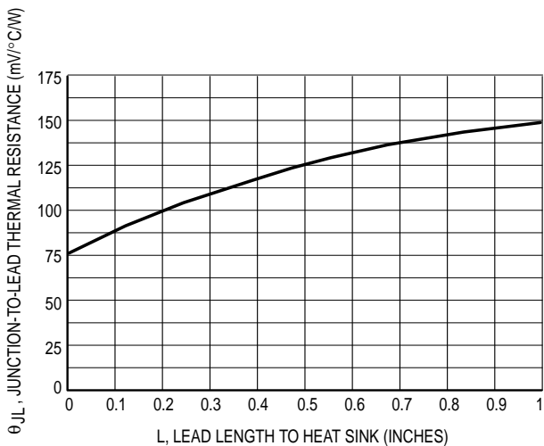
Figure 1. Typical Thermal Resistance versus Lead Length
