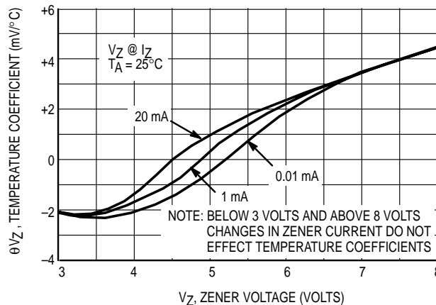
Figure 2. Effect of Zener Current
