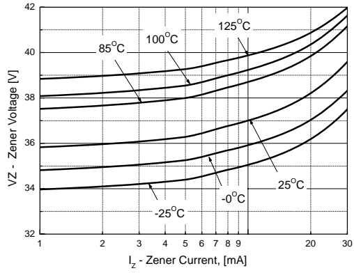
Figure 7. MM3Z36VB Zener current vs. Zener Voltage
