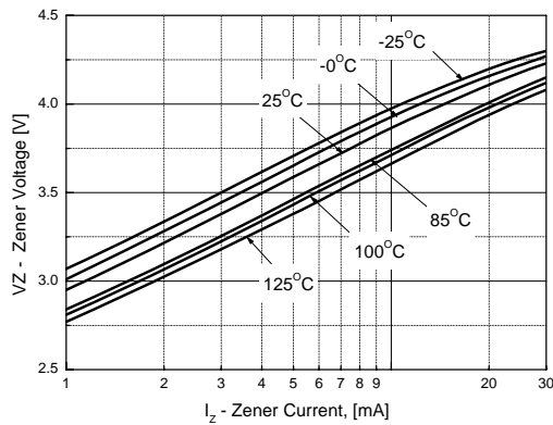
Figure 3. MM3Z3V6B Zener current vs. Zener Voltage
