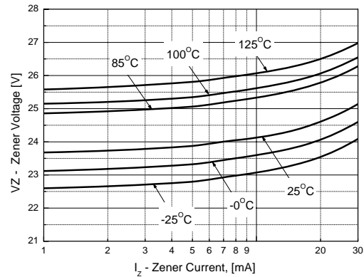
Figure 6. MM3Z24VB Zener current vs. Zener Voltage
