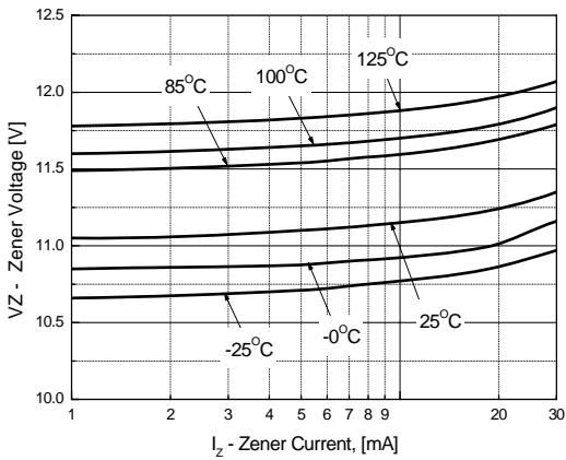
Figure 5. MM3Z11VB Zener current vs. Zener Voltage
