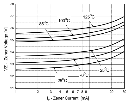
Figure 6. MM3Z24VB Zener current vs. Zener Voltage
