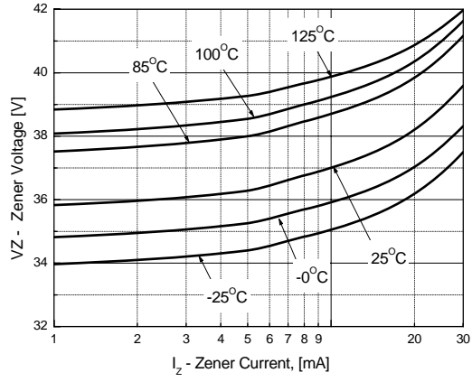
Figure 7. MM3Z36VB Zener current vs. Zener Voltage
