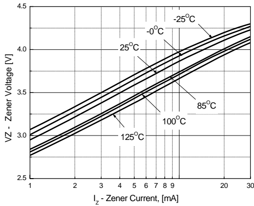
Figure 3. MM3Z3V6B Zener current vs. Zener Voltage
