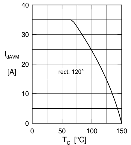
Fig. 4 Maximum forward current at case temperature T_C
