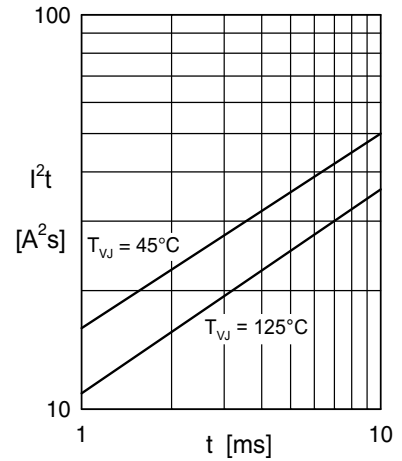
Fig. 2 I^2t versus time (1-10 ms) per diode
