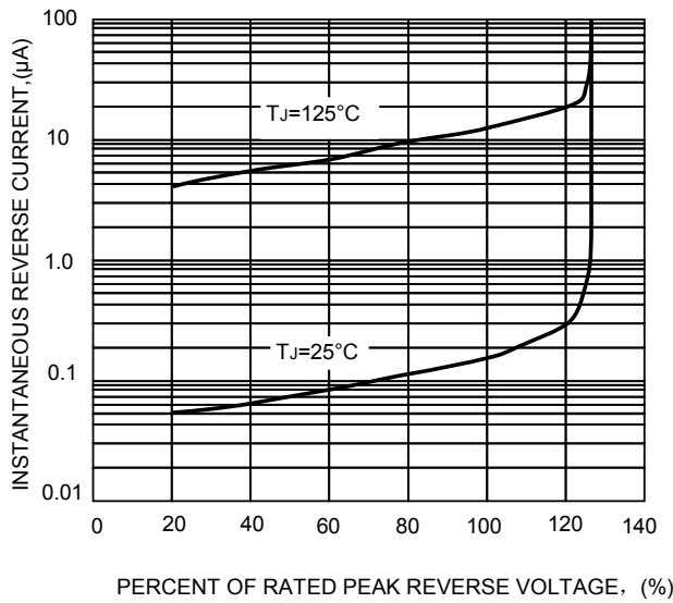
FIG.3-TYPICAL REVERSE CHARACTERISTICS
