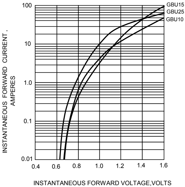
FIG.3-TYPICAL FORWARD CHARACTERISTICS
