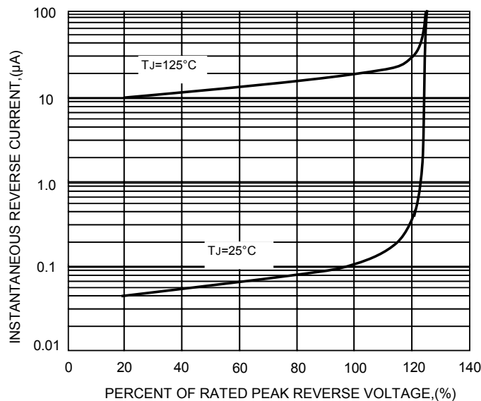
FIG.5-TYPICAL REVERSE CHARACTERISTICS
