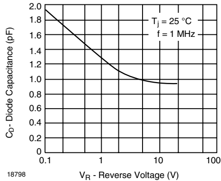
Figure 1. Diode Capacitance
