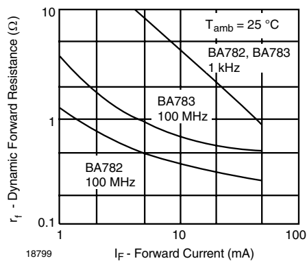
Figure 2. Dynamic Forward Resistance vs. Forward Current
