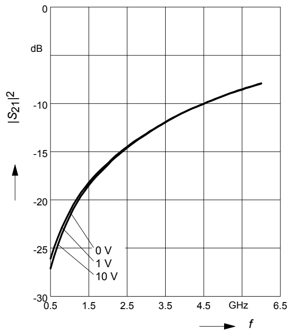
Isolation I_{SO} = -|S_{21}|^2 = f(f) V_R = Parameter BAR64-02LRH in series configuration, Z = 50\Omega
