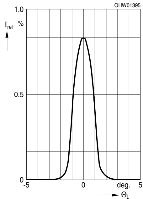
Farfield Distribution Perpendicular to Junction I_{rel} vs. \theta_{\perp}
