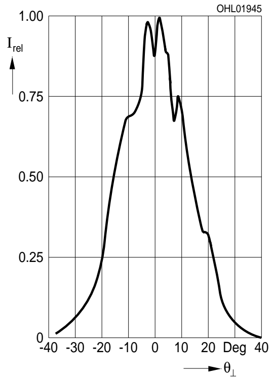
Far-field distribution perpendicular to junction I_{rel} vs. angle \theta_{\perp}
